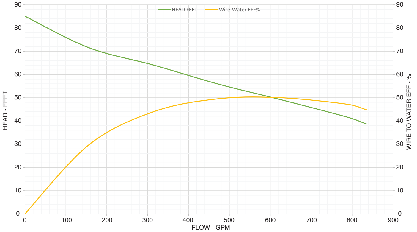
PERFORMANCE CURVE
